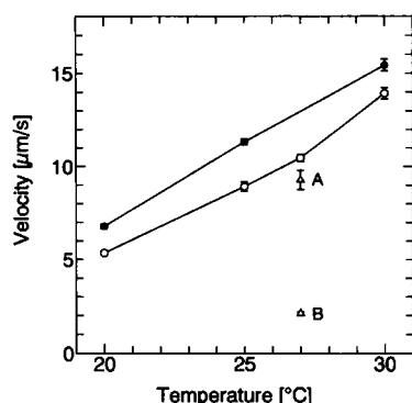
FIGURE 4 Dependence of the sliding velocity on the temperature. The velocities are plotted for myosin-LMM copolymers sliding along actin filaments ( \circ ) and the actin-tropomyosin complexes ( \bullet ). The bar represents the standard error of the mean for 30–43 copolymers. Medium: 36 mM KCl, 29 mM \text{MgCl}_2 , 1.7 mM ATP, 19 mM HEPES, pH 7.8, and the oxygen-reduction system. The length of myosin filaments used was 2–4 \mu\text{m} . The velocities of actin along myosin-rod copolymer filaments in the normal direction ( \triangle , A) and the opposite direction ( \triangle , B) obtained in the same solution (Yanagida et al., in press) are also shown.
