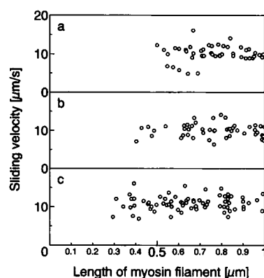
FIGURE 7 Sliding velocities of myosin-LMM copolymer of various lengths on the actin filament. Medium: 36 mM KCl, 29 mM \text{MgCl}_2 , 1.7 mM ATP, 19 mM HEPES, pH 7.8, the oxygen-reduction system and 0% ( a ), 0.1% ( b ), 0.3% ( c ) methylcellulose. The temperature was 27 \pm 1^\circ\text{C} .
