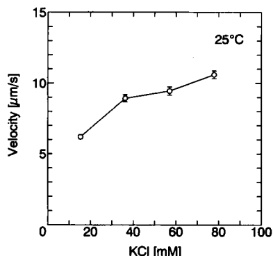
FIGURE 5 Dependence of the sliding velocity on ionic strength. The ionic strength was adjusted by changing the concentration of KCl in a solution containing 2.9 mM \text{MgCl}_2 , 1.7 mM ATP, 19 mM HEPES, pH 7.8, and the oxygen-reduction system. The bar gives the standard error of the mean for 34–39 copolymers. The temperature was 25 \pm 1^\circ\text{C} . The length of myosin filaments was 2–4 \mu\text{m} .
